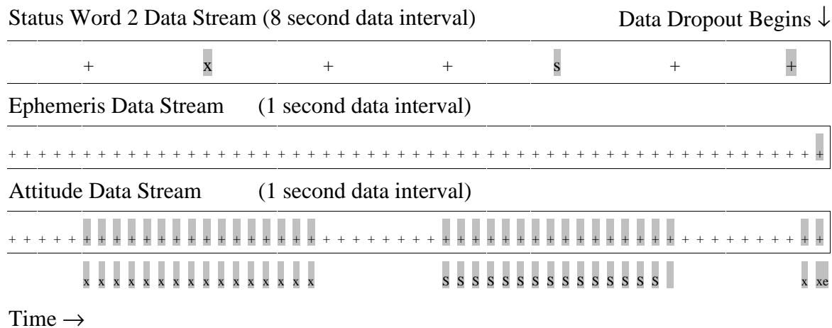
Figure 1-2. Status Word 2 and Ephemeris Influence on Attitude Flagging
